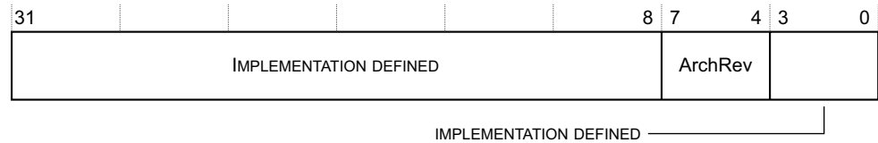
Figure 12-2 GICD_PIDR2 bit assignments
